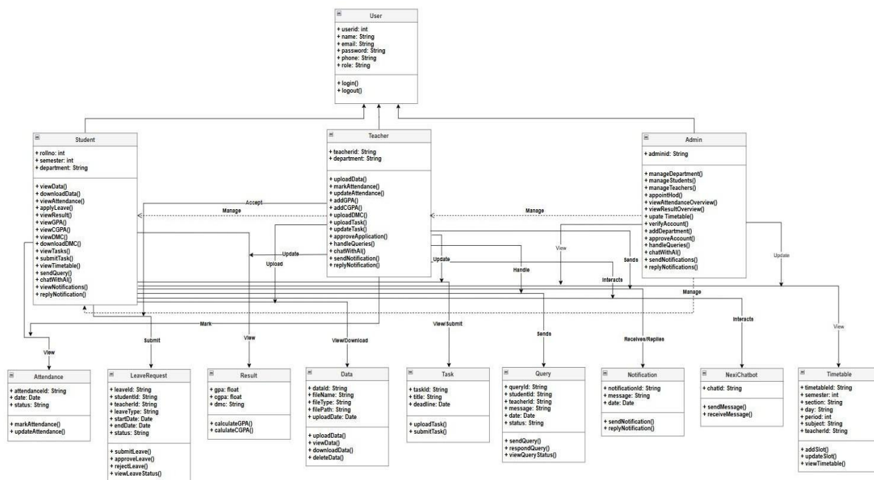
Figure 5.3: Class Diagram
